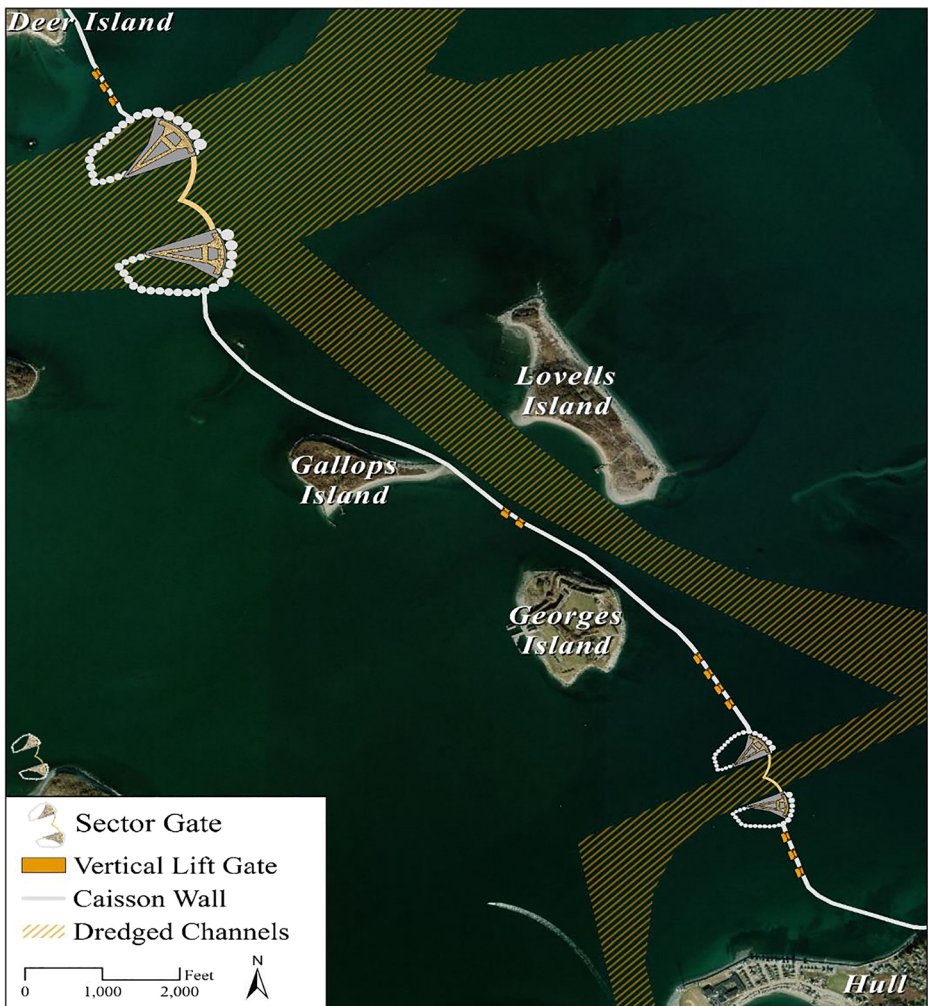
Fig. 2 Outer harbor barrier configuration. (1 ft = 0.3048 m). From Kirshen et al. (2018)
